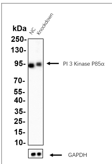
Western blot analysis of lysates from HL60 WT and knockdown cell. Cell lysates were separated by 4-20% SDS-PAGE, and the membrane was blotted with PI3-Kinase p85 α (PT0082R) rabbit mAb. The HRP-conjugated Goat anti-Rabbit IgG (H + L) antibody was used to detect the antibody.
