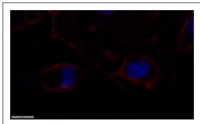
Immunofluorescence analysis of MCF7 cell. 1,primary Antibody was diluted at 1:100(4°C overnight). 2, Goat Anti Rabbit IgG (H&L) - AFluor 594 Secondary antibody(catalog No: RS3611) was diluted at 1:500(room temperature, 50min).
