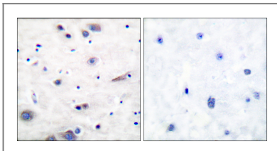
Immunohistochemistry analysis of paraffin-embedded human brain, using SHP-2 (Phospho-Tyr580) Antibody. The picture on the right is blocked with the phospho peptide.
