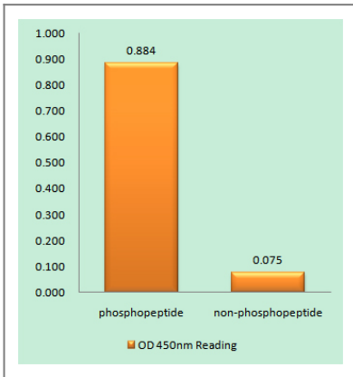
Enzyme-Linked Immunosorbent Assay (Phospho-ELISA) for Immunogen Phosphopeptide (Phospho-left) and Non-Phosphopeptide (Phospho-right), using SHP-2 (Phospho-Tyr580) Antibody
