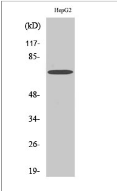
Western Blot analysis of various cells using Phospho-SH-PTP2 (Y580) Polyclonal Antibody
